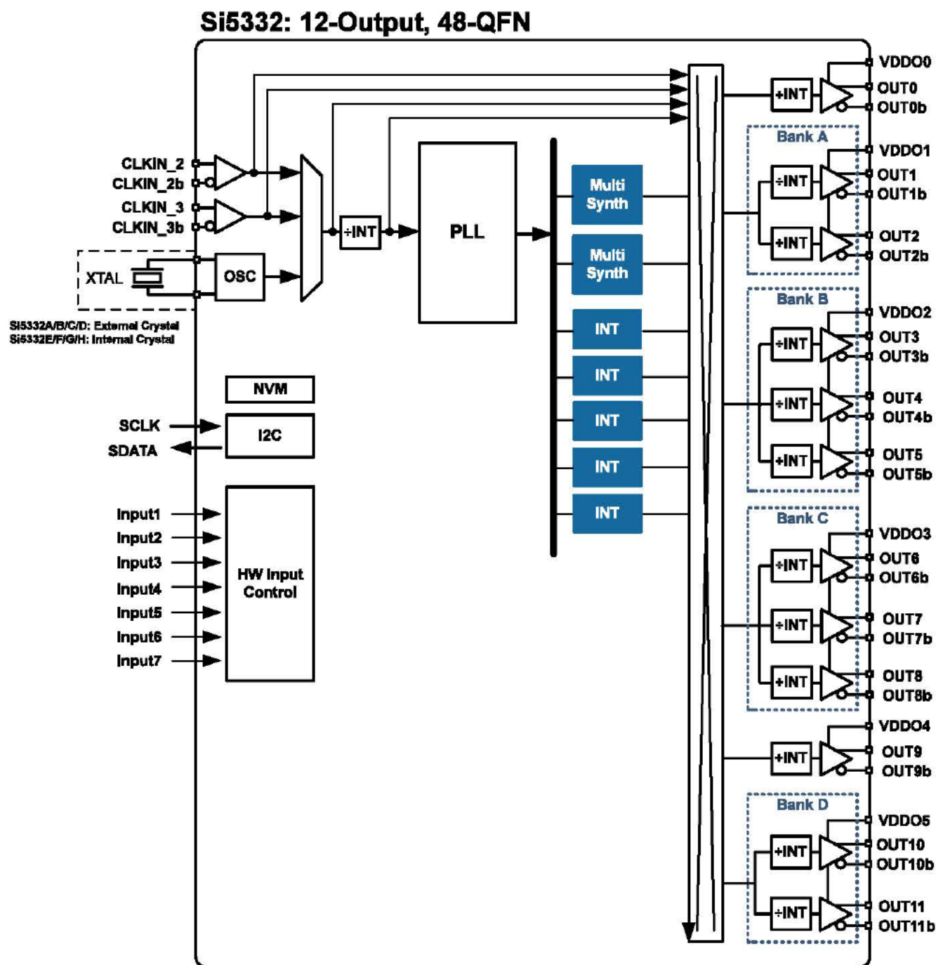
Figure 3.1. Block Diagram for 12-Output Si5332 in 48-QFN
