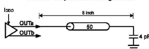
LVCMOS Output Test Configuration
