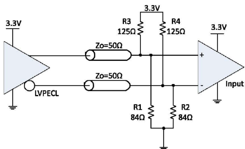
Figure 3.8. 3.3 V LVPECL Output Termination, Option 2
