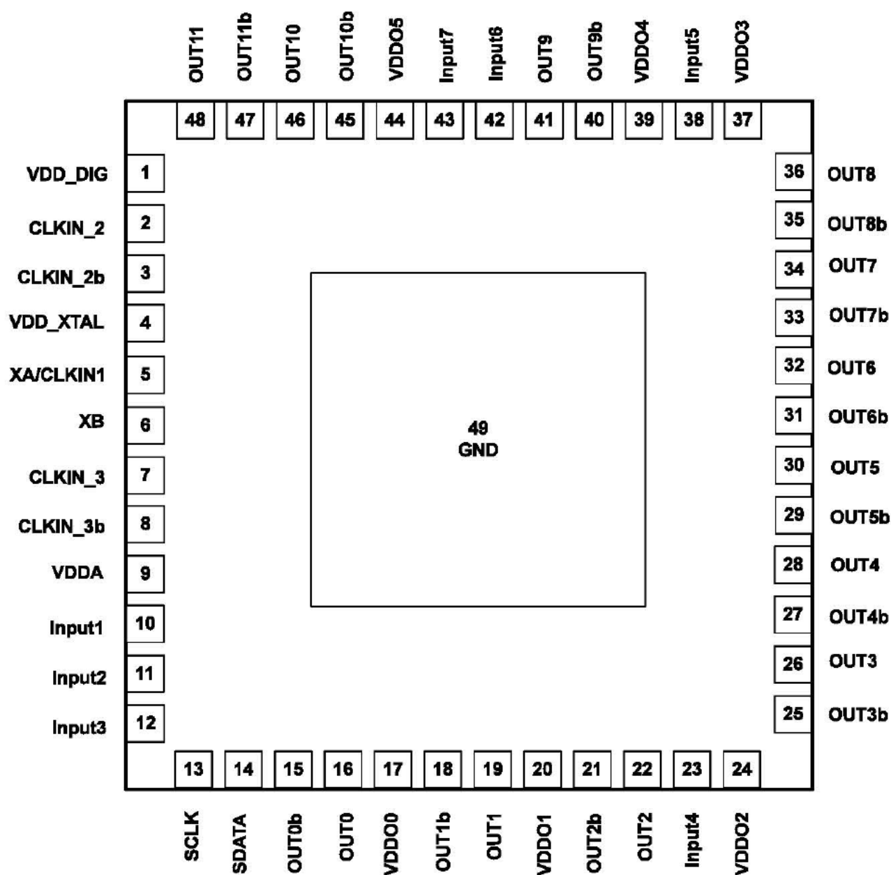
Figure 6.1. 48-QFN
